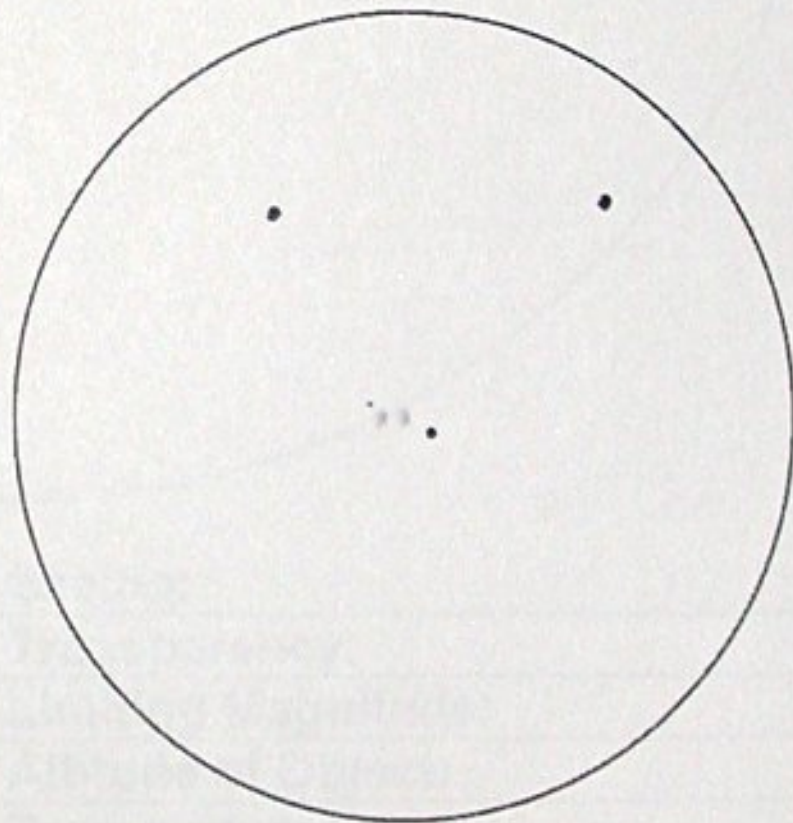
30" f/4.3 reflector @ 1256x Field: 2.9'
